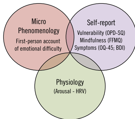
Figure 1 • Methodological framework studying change through mindfulness practice, incorporating vulnerability. ECG-HRV: Heart Rate Variability, OPD-SQ: Structure Questionnaire, BDI: Beck Depression Inventory, OQ45: Outcome Questionnaire, FFMQ: Five-Facet Mindfulness Questionnaire).
